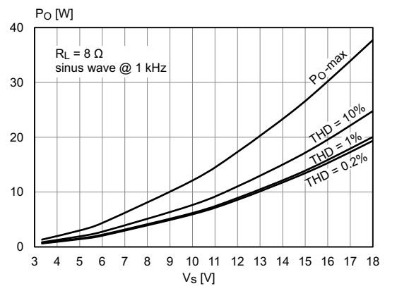
Figure 24. Output power vs. supply voltage ( R_L = 8\ \Omega , sine wave)
