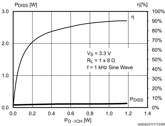
Figure 20. Efficiency and power dissipation ( V_S = 3.3\text{ V} , R_L = 1 \times 8\ \Omega , f = 1\text{ kHz} sine wave)
