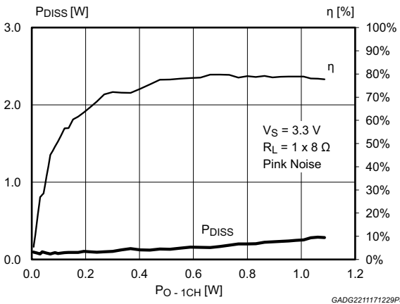
Figure 21. Efficiency and power dissipation ( V_S = 3.3\text{ V} , R_L = 1 \times 8\ \Omega , f = 1\text{ kHz} pink noise)
