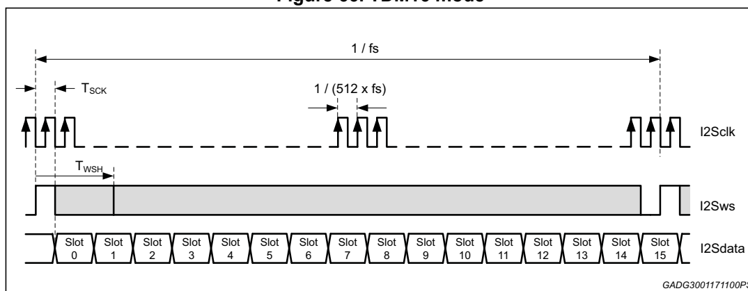
Figure 66. TDM16 mode
