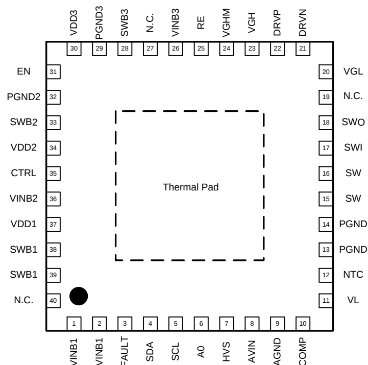
Figure 2. Pin Configuration
