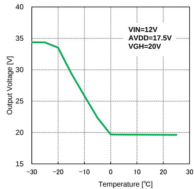
Figure 32. VGH Voltage vs Ta
