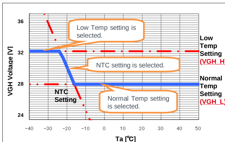
Figure 42. VGH thermal compensation
