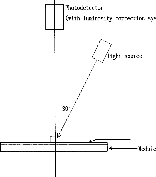
Measuring method (b) for optical characteristics
