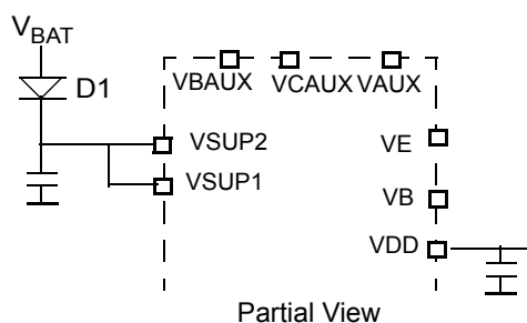
ex 4: No External Transistor - No VAUX
