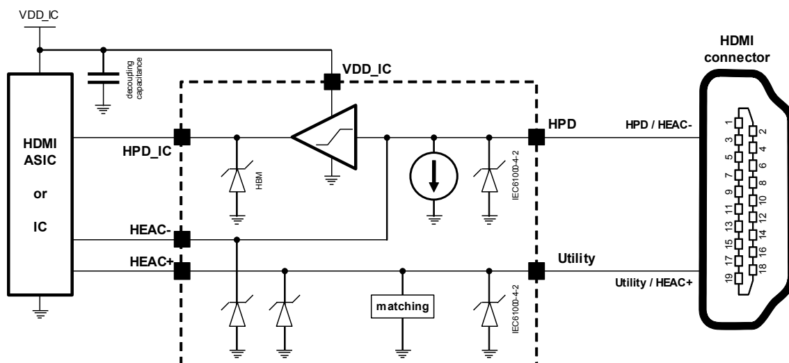
Figure 7. HEAC / HPD utility functional block diagram
