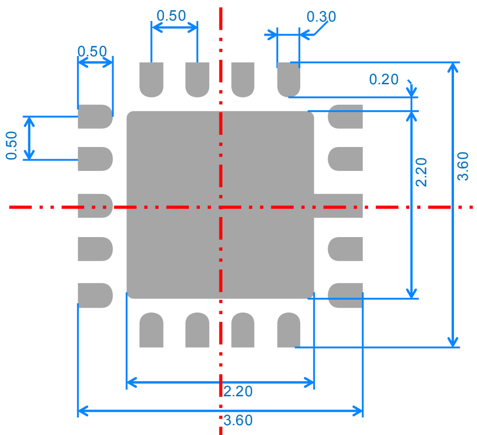
Figure 19. QFN footprint recommendation (dimensions in mm)
