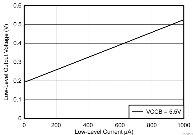
V_{CCA} = 3.0V V_{IL(A)} = 0.15V Figure 7-2. Low-Level Output Voltage ( V_{OL(Bx)} ) vs Low-Level Current ( I_{OL(Bx)} )
