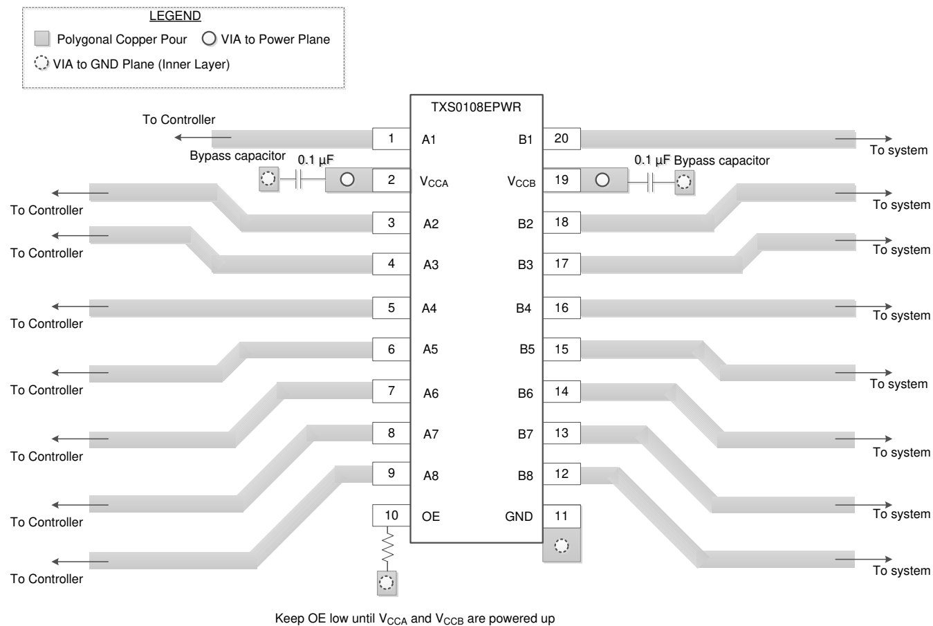
Figure 10-3. Layout Example
