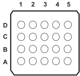
Figure 5-1. ZXY PACKAGE 20 BUMP (BOTTOM VIEW)
