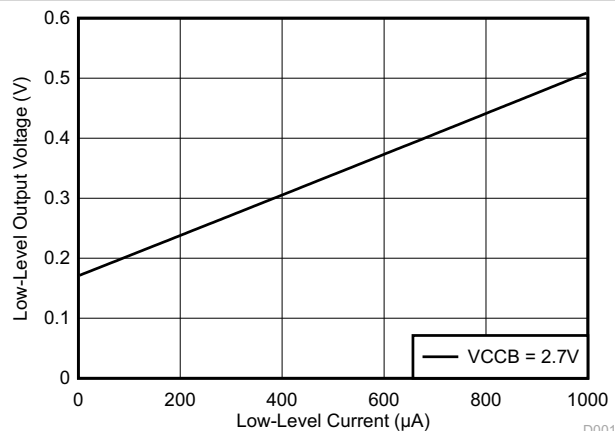
V_{CCA} = 2.3V V_{IL(A)} = 0.15V Figure 7-1. Low-Level Output Voltage ( V_{OL(Bx)} ) vs Low-Level Current ( I_{OL(Bx)} )
