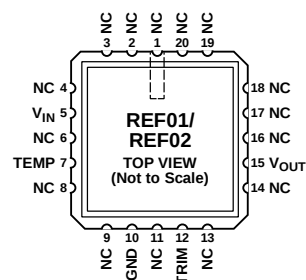
Figure 3. 20-Terminal LCC (RC-Suffix; 883 Parts Only)
