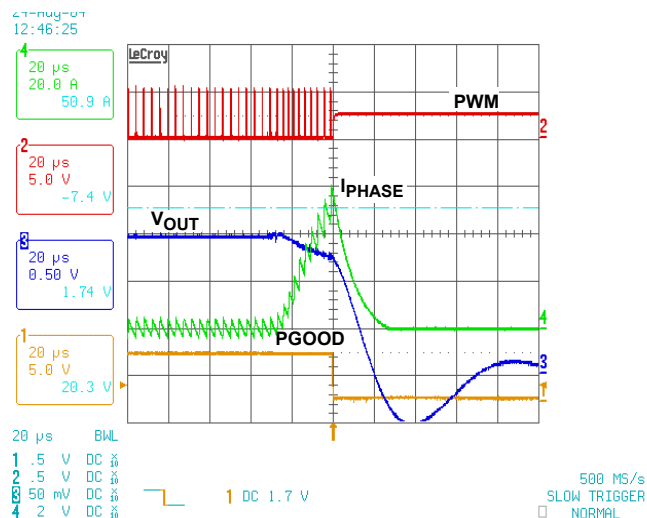
FIGURE 29. WOC - SHORT CIRCUIT PROTECTION
