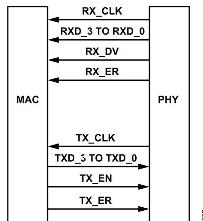
Figure 10. MII MAC PHY Interface Signals
