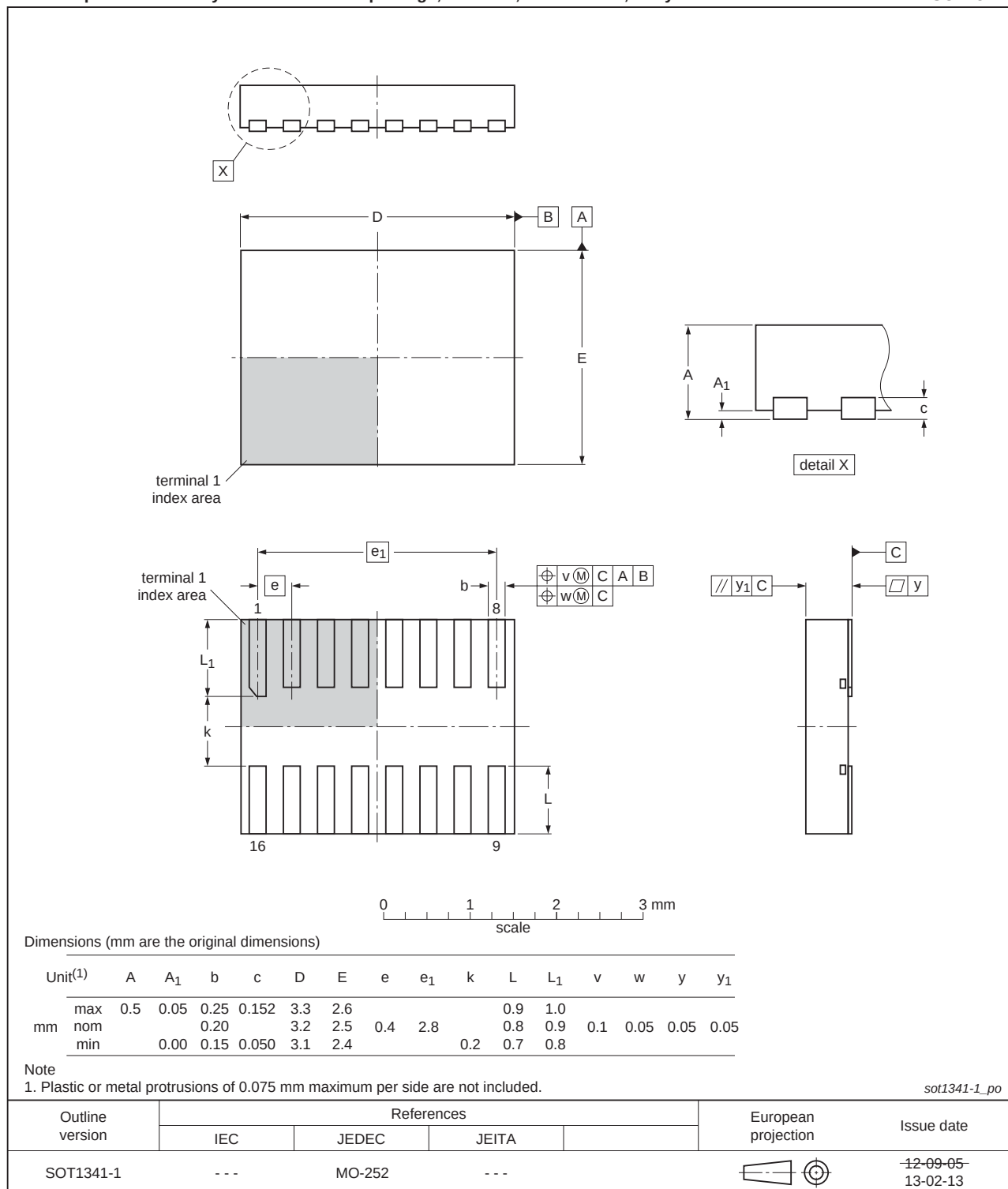
Fig 41. Package outline SOT1341-1 (XSON16)
