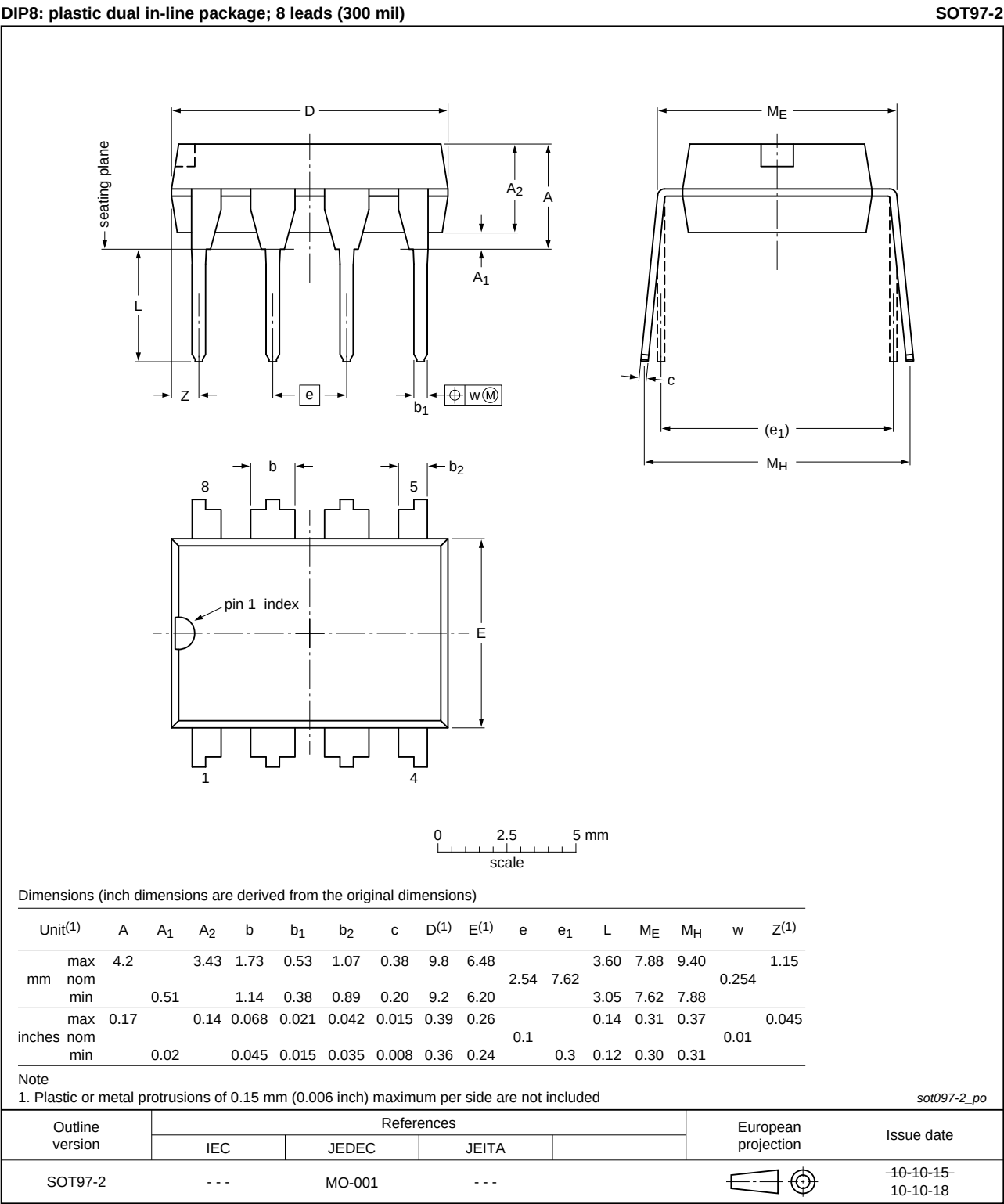
Fig 37. Package outline SOT097-2 (DIP8)
