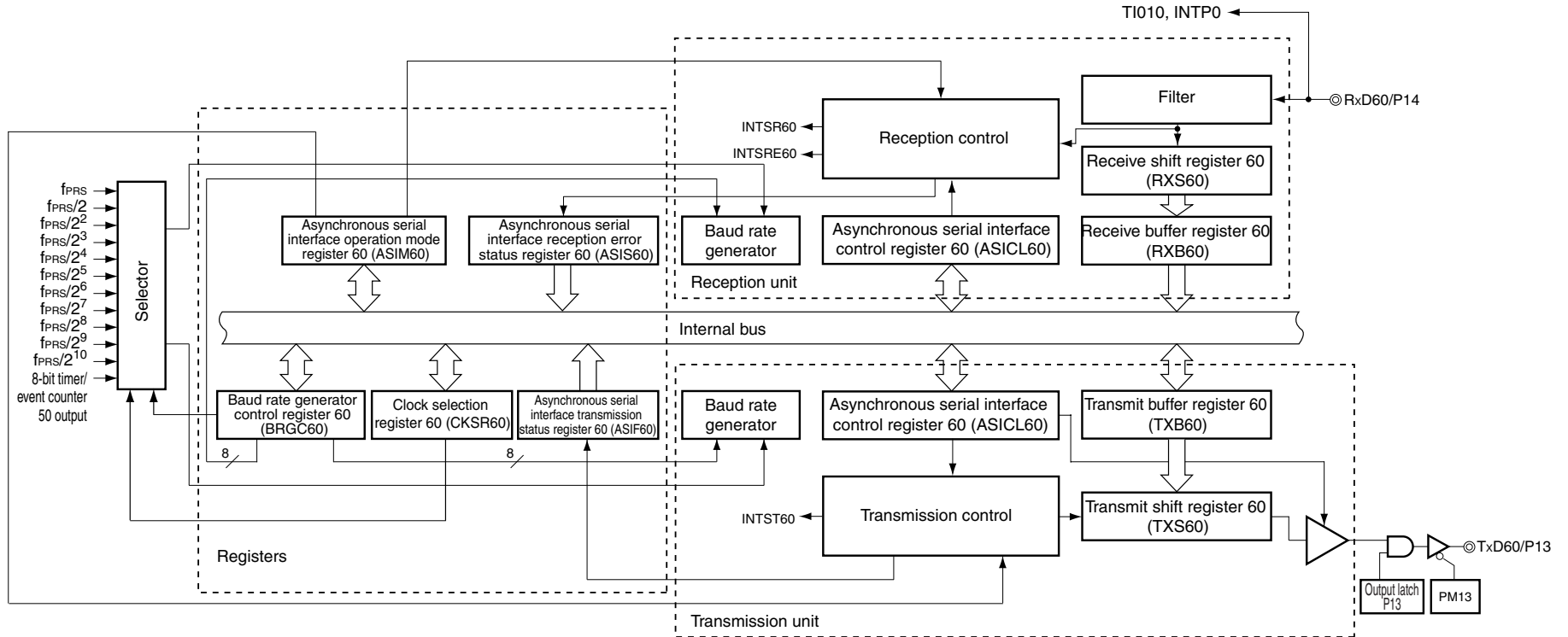
Figure 13-5. Block Diagram of Serial Interface UART60
