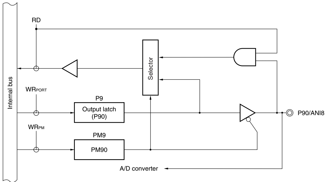
Figure 4-16. Block Diagram of P90
