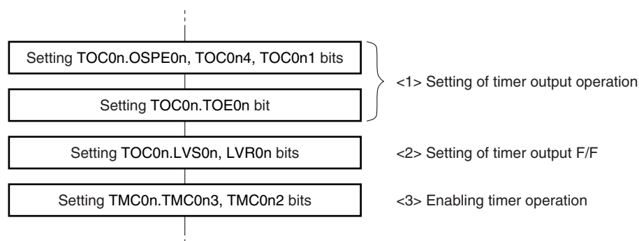
Figure 6-42. Example of Flow for Setting LVS0n and LVR0n Bits
