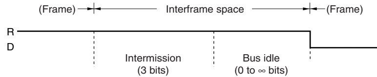
Figure 15-13. Interframe Space (Error Active Node)
