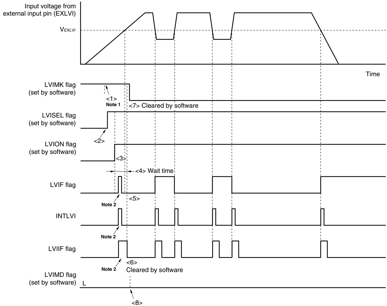
Figure 21-8. Timing of Low-Voltage Detector Interrupt Signal Generation (Detects Level of Input Voltage from External Input Pin (EXLVI))
