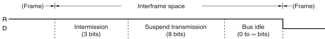
Figure 15-14. Interframe Space (Error Passive Node)
