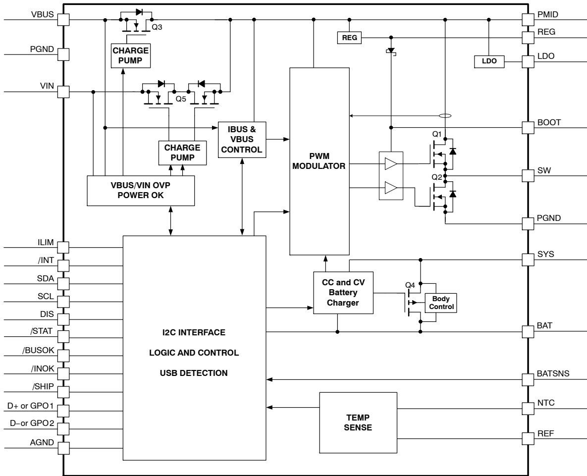
Figure 5. Block Diagram
