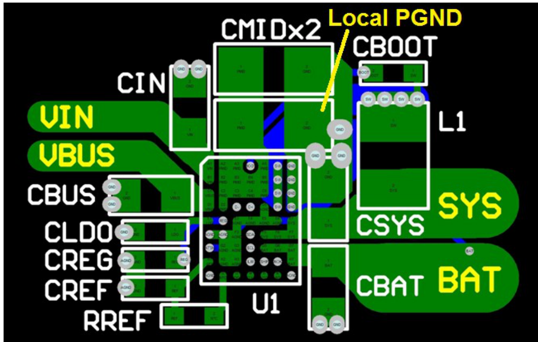
Figure 55. Recommended Component Placement and Routing
