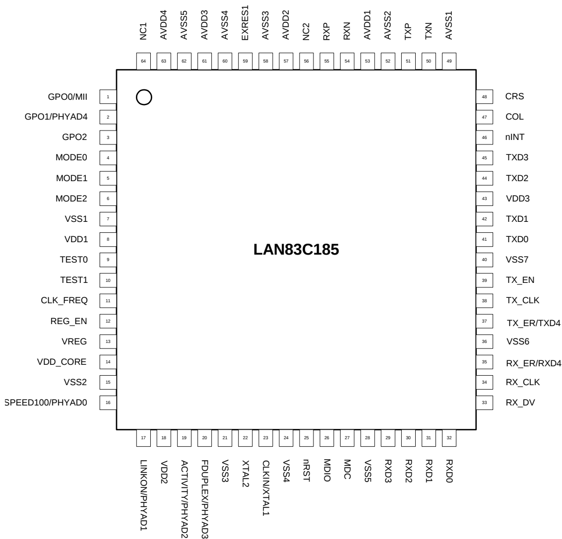
Figure 2.1 Package Pinout
