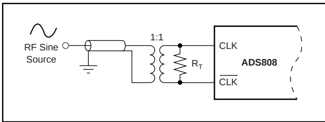
FIGURE 12. Applying a Sinusoidal Clock to the ADS808.
