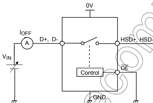
Figure 8: Power off Leakage Current
