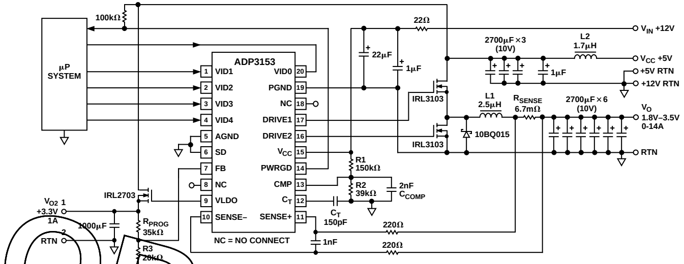
Figure 2. Typical VFM8.2 Compliant Core DC/DC Converter Circuit
