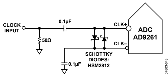
Figure 43. Single-Ended Clock
