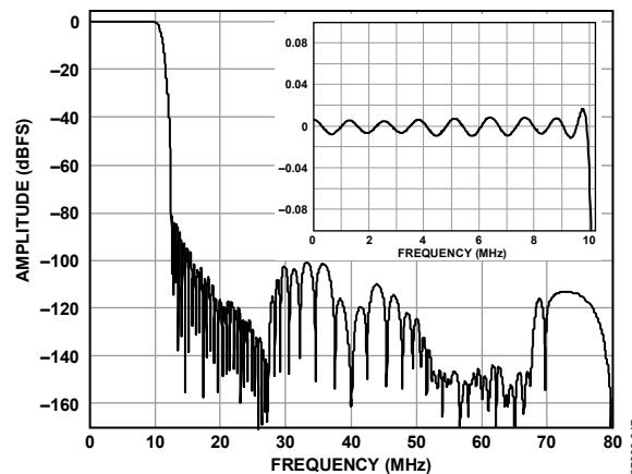
Figure 47. 10 MHz Signal Bandwidth, 160 MSPS
