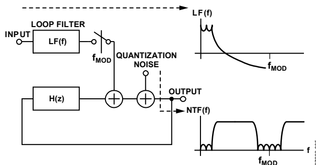
Figure 35. Continuous Time Converter
