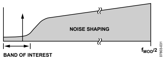
Figure 31. Noise Shaping
