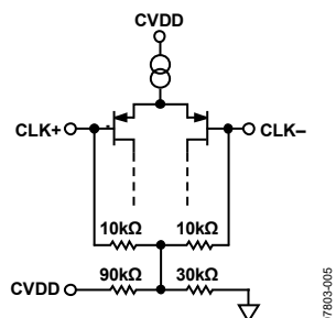
Figure 23. Equivalent Clock Input Circuit
