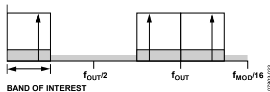
Figure 33. Sample Rate Converter
