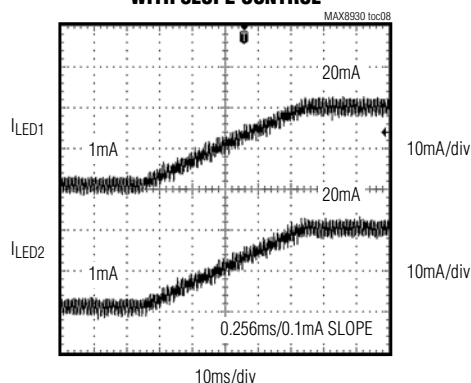
WLED—DIMMING CURRENT TRANSIENT WITH SLOPE CONTROL
