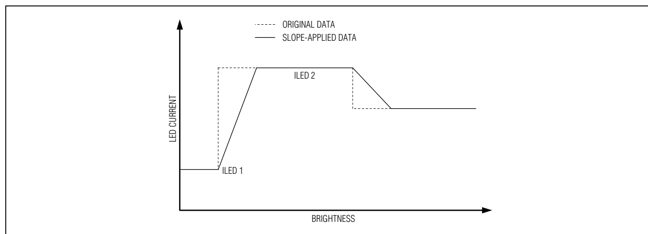
Figure 6. LED Current vs. Brightness
