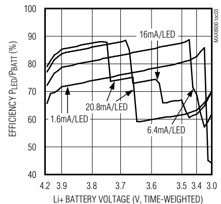
EFFICIENCY vs. Li+ BATTERY VOLTAGE DRIVING 6 MATCHED LEDs
