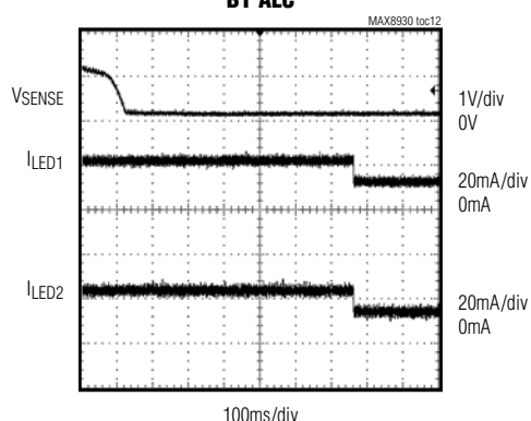
WLED—DIMMING CURRENT TRANSIENT BY ALC
