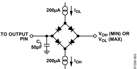
Figure 5. Load Circuit for SDO Timing Diagram
