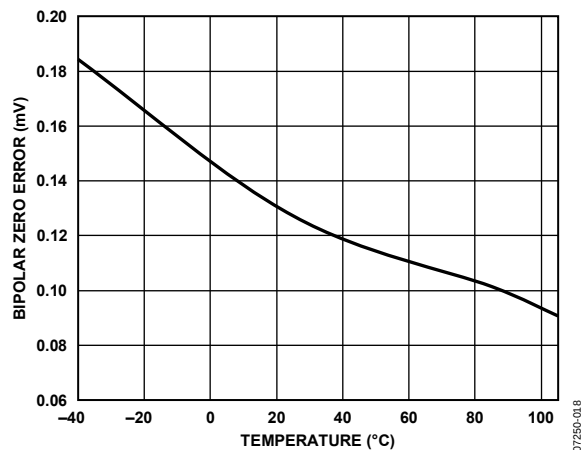
Figure 13. Bipolar Zero Error vs. Temperature
