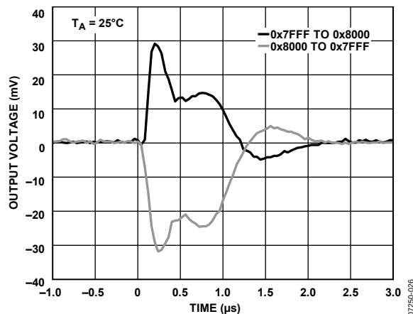
Figure 20. Major Code Transition Glitch Energy
