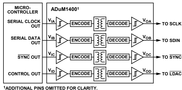
Figure 30. Isolated Interface
