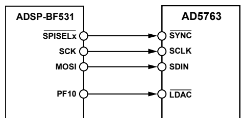
Figure 31. AD5763 to Blackfin Interface
