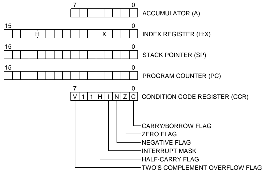
Figure 6-1. CPU registers
