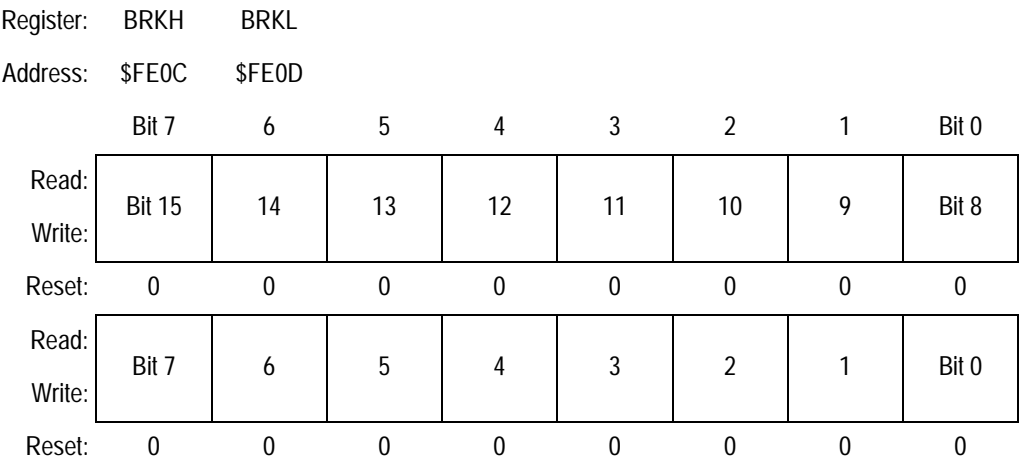
Figure 11-4. Break Address Registers (BRKH and BRKL)
