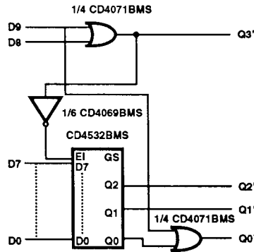
FIGURE 12. 0-TO-9 KEYBOARD ENCODER
