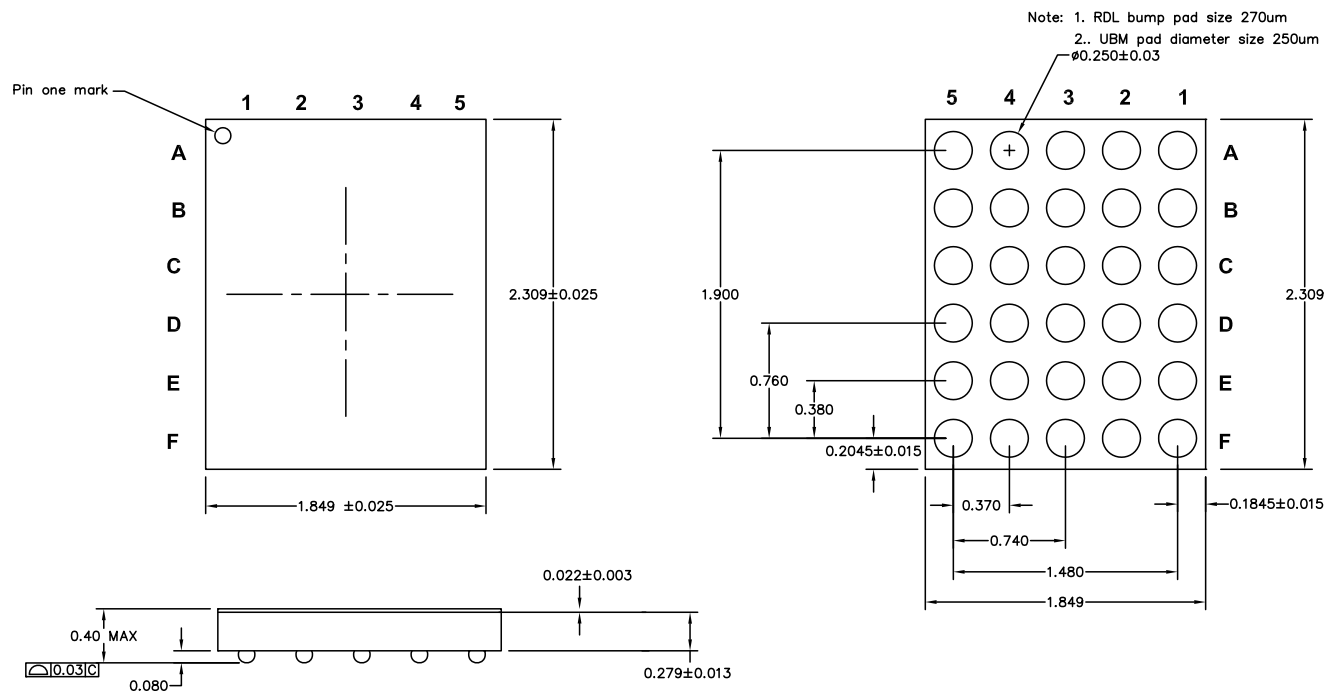
Figure 21. 30-Ball WLCSP (1.85 × 2.31 × 0.40 mm) Package Outline, 001-44613
