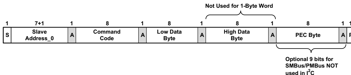
Figure 25. Write Byte/Word Protocol
