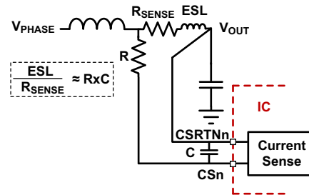
Figure 11. Sense Resistor in Series with Inductor
