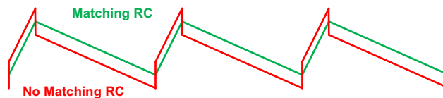
Figure 12. Voltage Across R with and without RC
