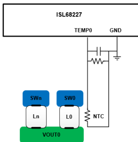
Figure 17. NTC Placement
