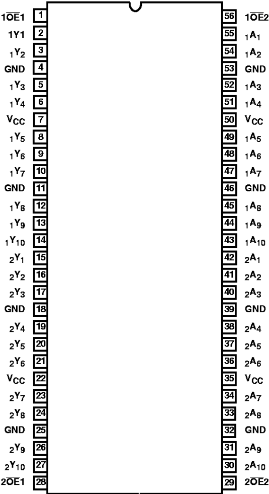
CD74FCT16827T, CD74FCT162827T, CD74FCT162H827T (SSOP, TSSOP) TOP VIEW
