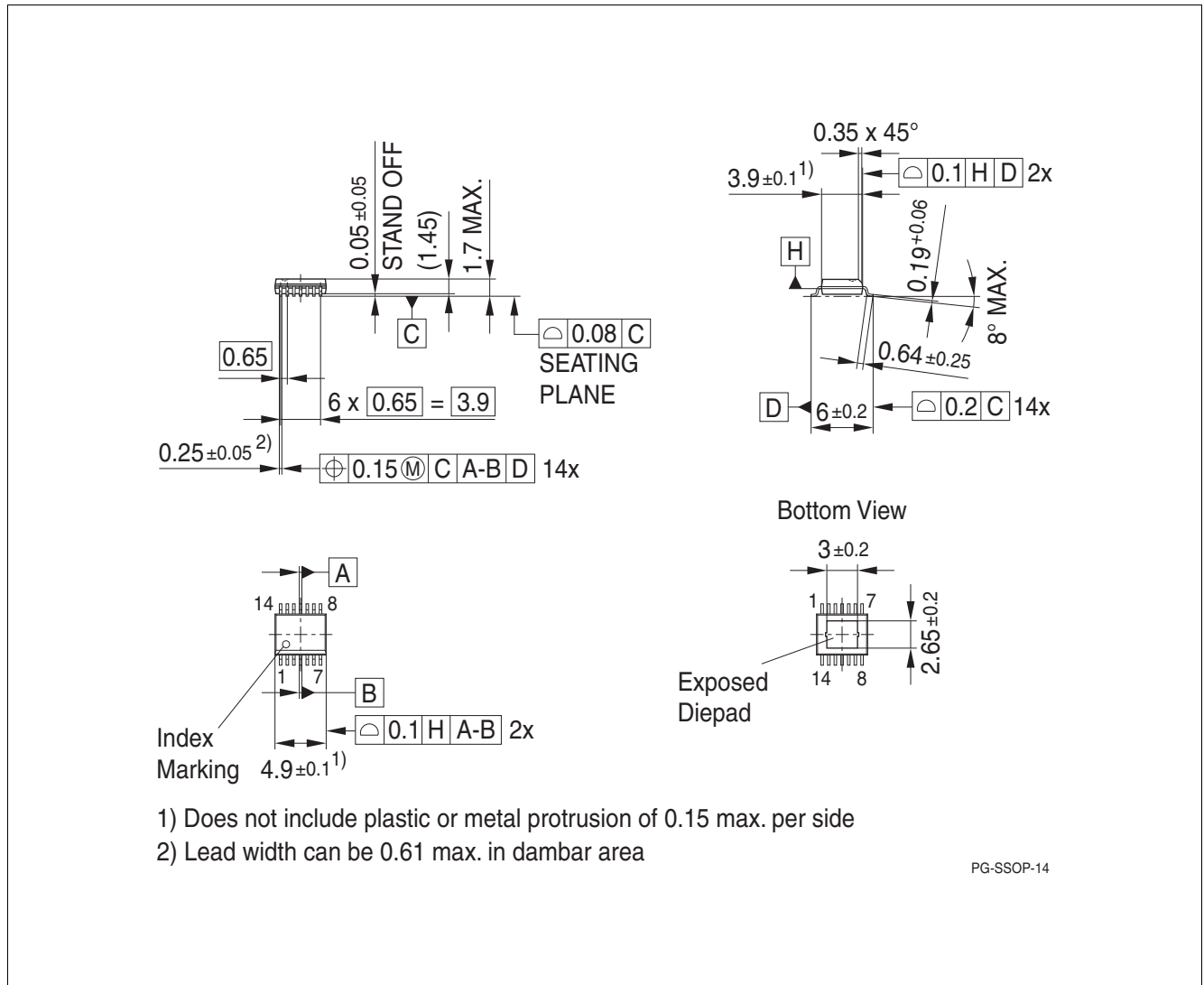
Figure 16 Outline PG-SSOP-14
