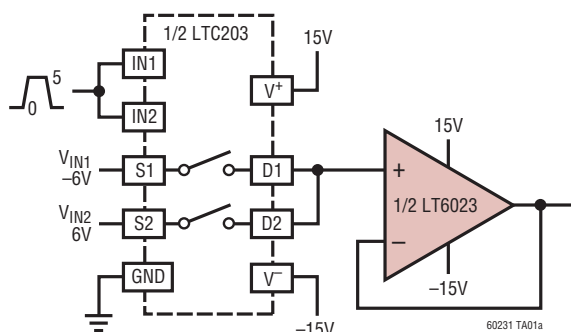
\pm 13.6 V Input Range MUX Buffer
