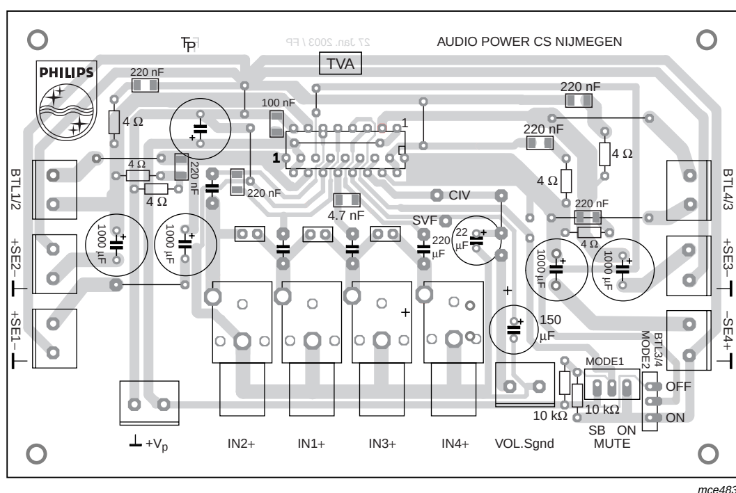
Fig 13. Printed-circuit board layout (single-sided); components view
