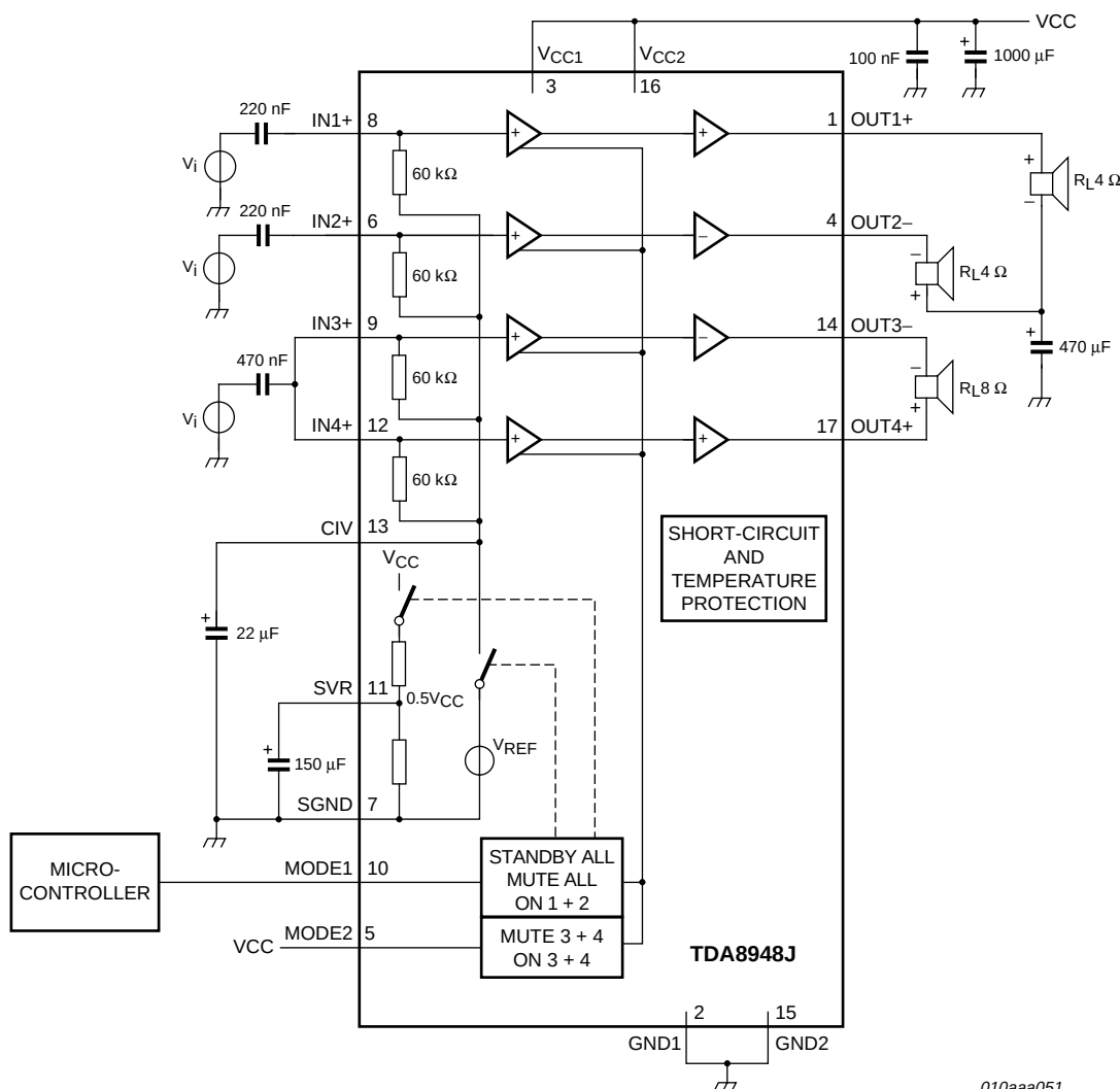
Fig 12. Application diagram with one pin control and reduction of capacitor
