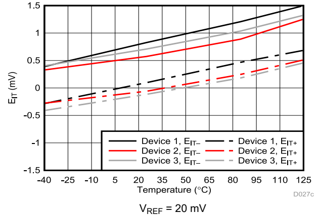
Figure 6-26. Cmp1 Trip Threshold Error vs Temperature
