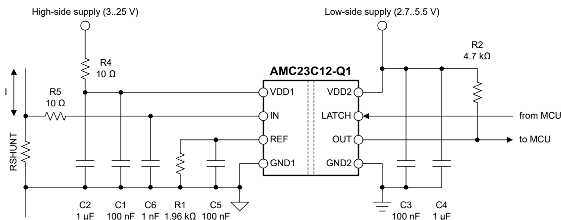
Figure 8-6. Decoupling of the AMC23C12-Q1
