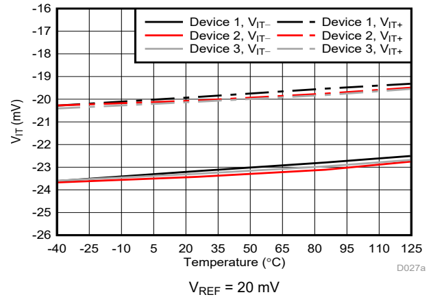
Figure 6-24. Cmp1 Trip Threshold vs Temperature
