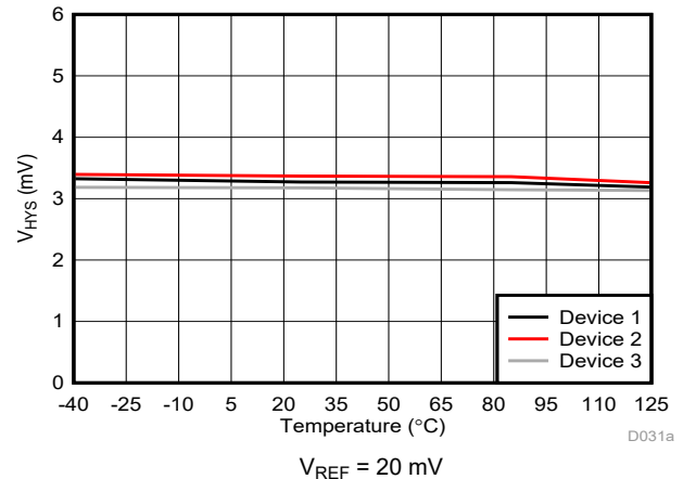
Figure 6-28. Cmp1 Trip Threshold Hysteresis vs Temperature
