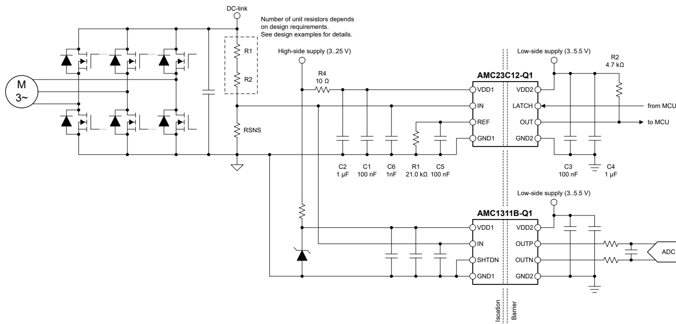
Figure 8-2. Using the AMC23C12-Q1 for Overvoltage Detection
