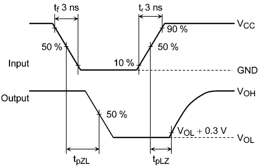
AC Waveform
