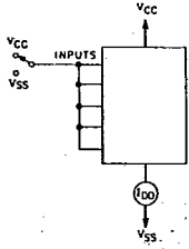
Fig. 13 — Quiescent device current test circuit.
