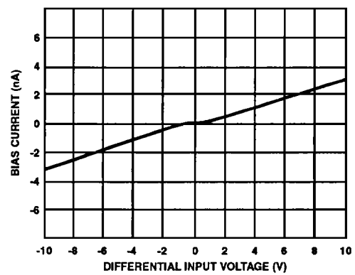
FIGURE 4. INPUT BIAS CURRENT vs DIFFERENTIAL INPUT VOLTAGE
