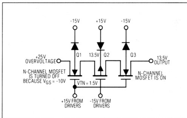
Figure 11. +25\text{V} Overvoltage Input to the ON Channel
