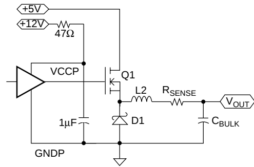
Figure 4. 12V Gate Bias Configuration
