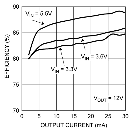
Power Efficiency vs. Output Current
