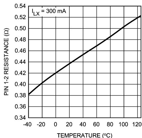
Pin 1-2 Resistance vs. Temperature
