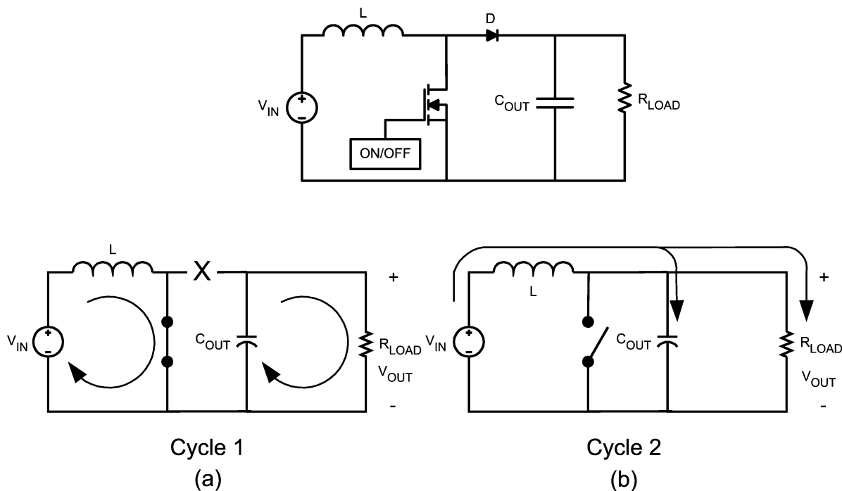
FIGURE 2. LM2707 Simplified Switching Circuit
