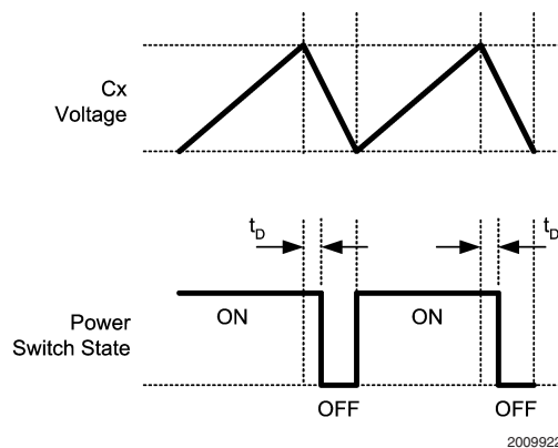
FIGURE 3. C_X Oscillator Waveform and Power Switch Operation
