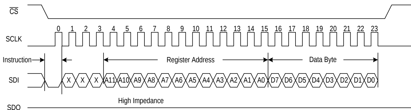
Figure-22 Write Operation In SPI Mode
