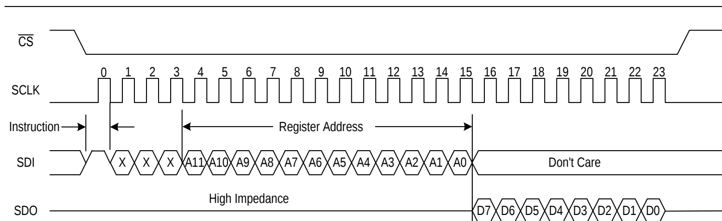
Figure-21 Read Operation In SPI Mode
