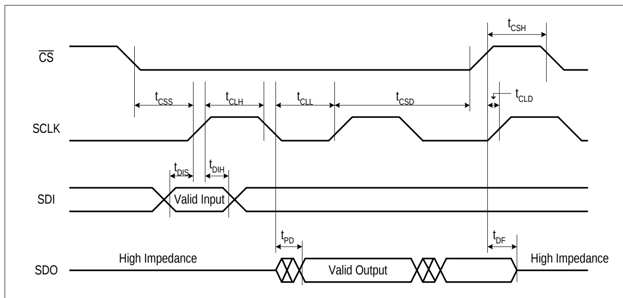
Figure-36 SPI Timing Diagram
