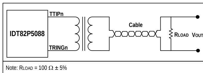
Figure-6 T1 Pulse Template Test Circuit
