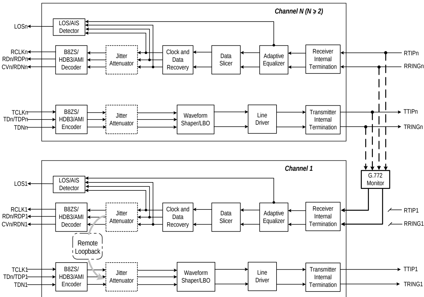
Figure-12 G.772 Monitoring Diagram
