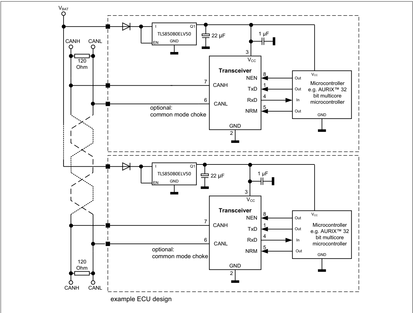
Figure 12 Application circuit
