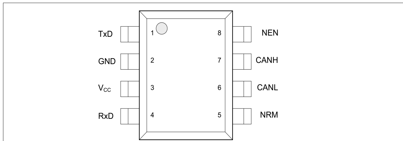
Figure 2 Pin assignment
