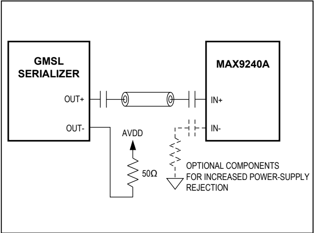
Figure 32. Coax-Mode Connection Diagram
