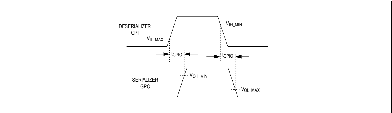
Figure 10. GPI-to-GPO Delay
