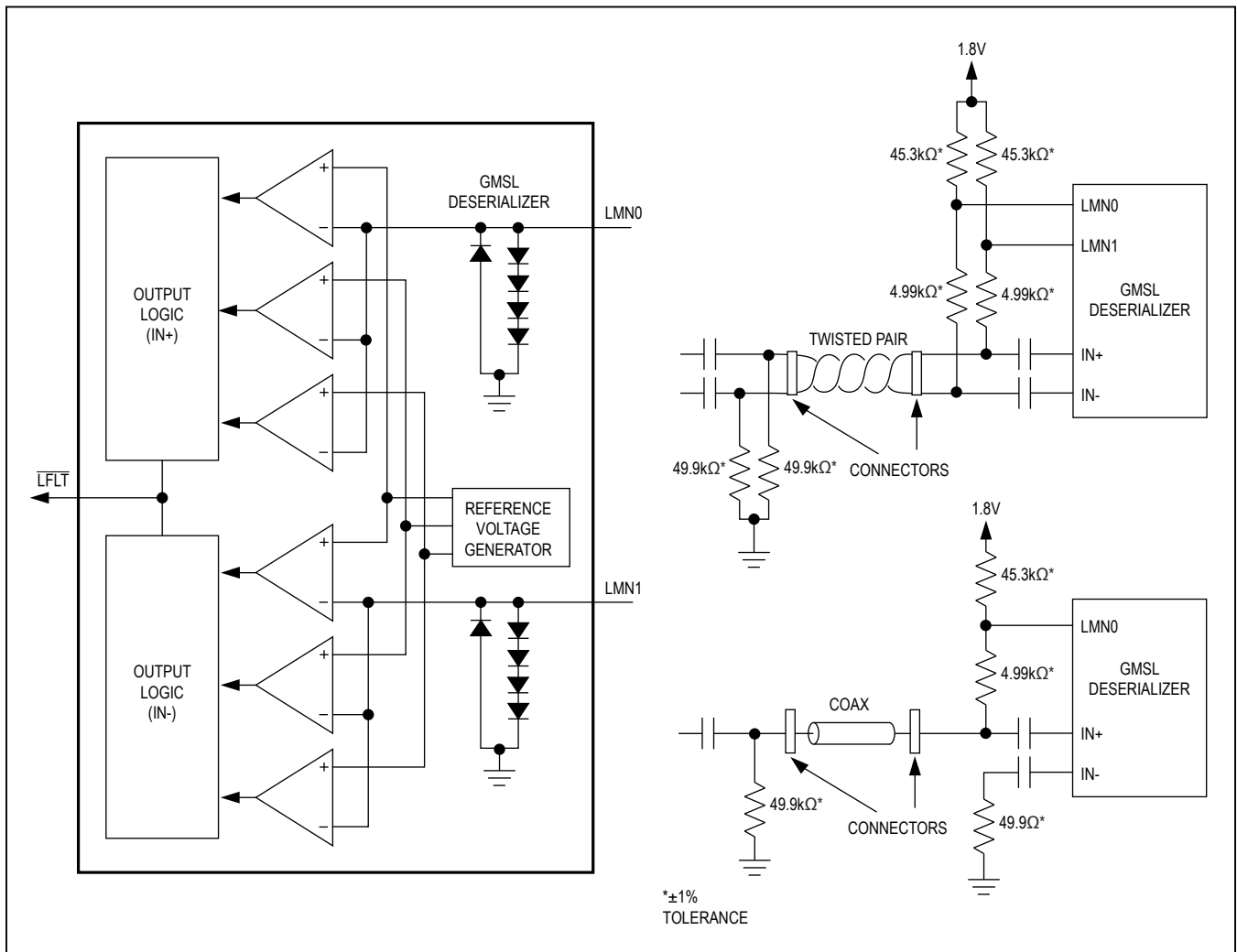
Figure 4. Line Fault
