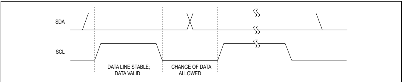
Figure 25. Bit Transfer
