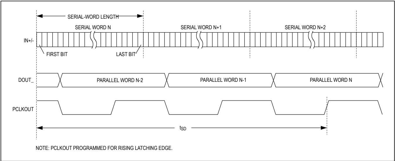
Figure 9. Deserializer Delay
