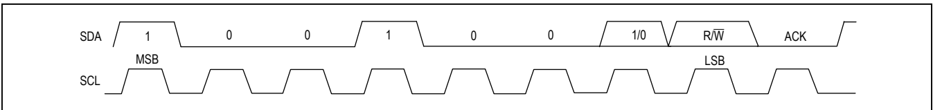
Figure 27. Slave Address
