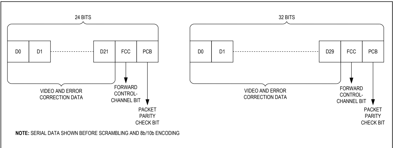
Figure 17. Serial-Data Format
