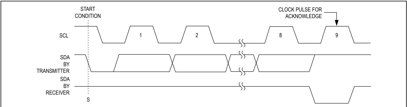
Figure 26. Acknowledge
