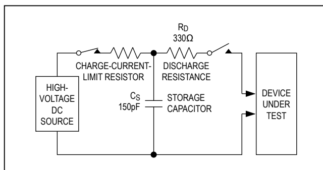
Figure 35 IEC 61000-4-2 Contact Discharge ESD Test Circuit
