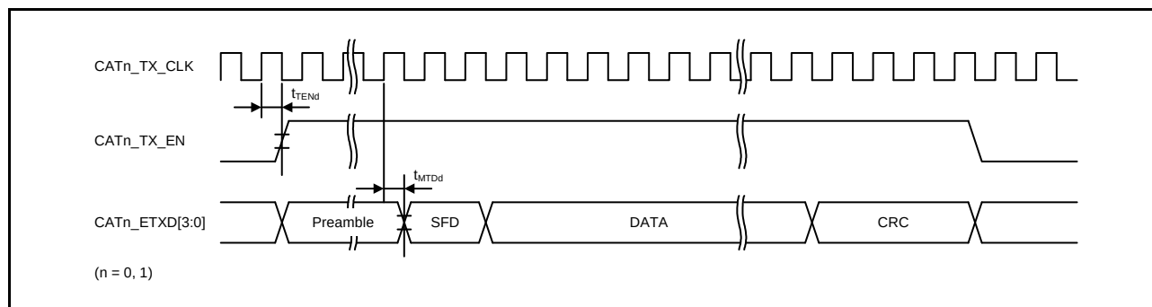
Figure 2.81 MII Transmission Timing (Normal Operation)
