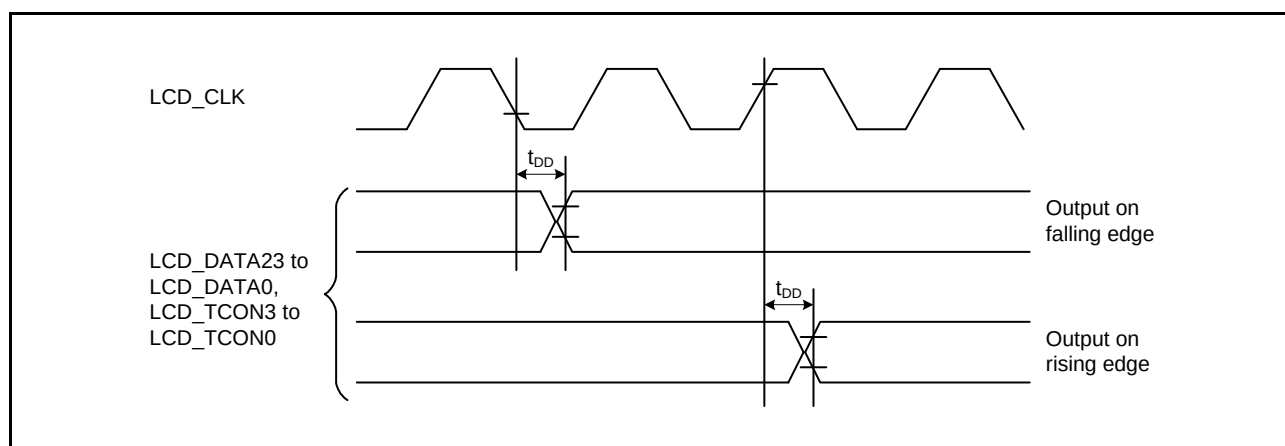
Figure 2.100 LCD Output Data Timing
