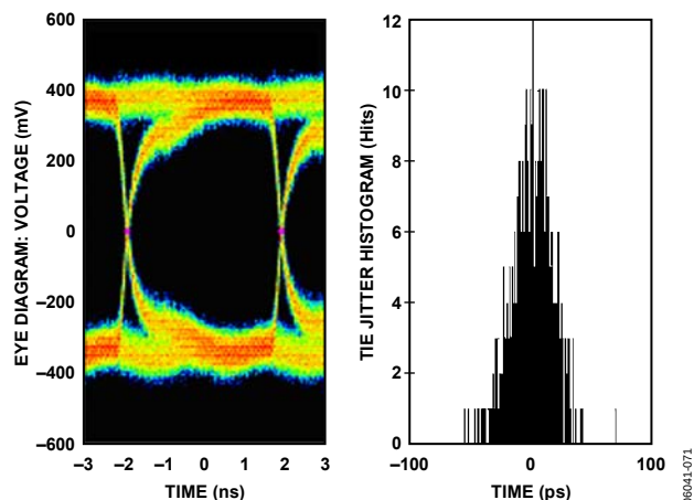
Figure 49. Data Eye for LVDS Outputs in ANSI Mode with Trace Lengths Greater than 24 Inches on Standard FR-4, AD9211-250
