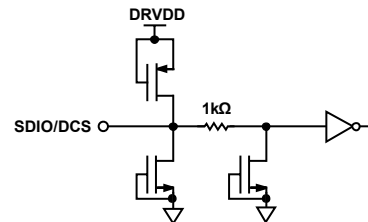
Figure 38. Equivalent SDIO/DCS Input Circuit
