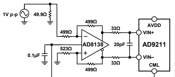
Figure 39. Differential Input Configuration Using the AD8138
