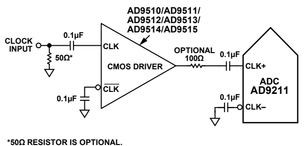
Figure 46. Single-Ended 3.3 V CMOS Sample Clock
