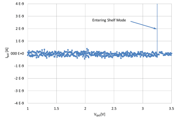
Figure 8. Battery leakage current vs. V_{BAT} ( V_{CHGIN} = 0 V; V_{BAT} < V_{BAT\_OVD} ; shelf mode)
