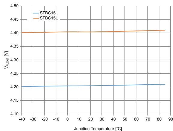
Figure 4. Floating voltage vs. temperature
