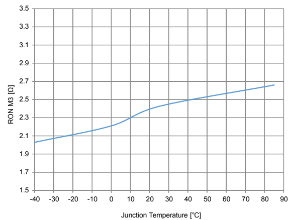
Figure 6. R_{ON} M3 vs. temperature
