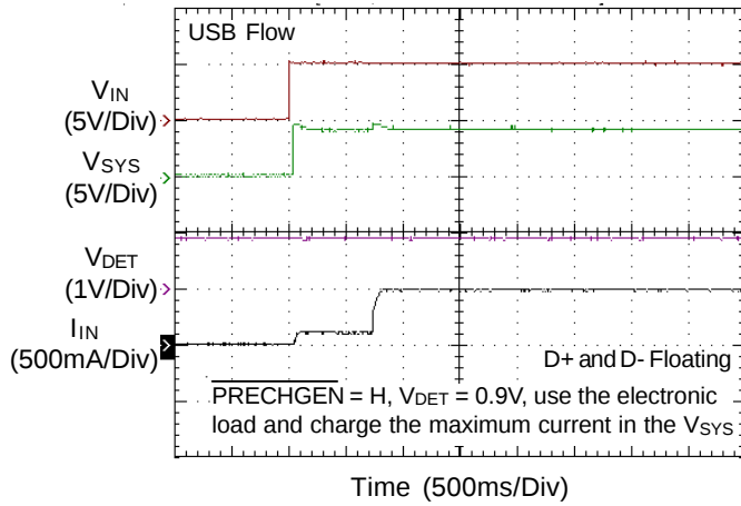
Standard 500mA Mode
