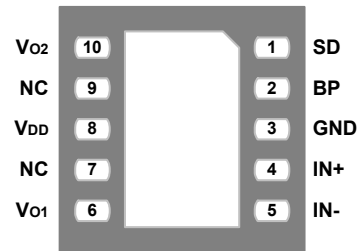
10MLP(BOTTOM VIEW)
