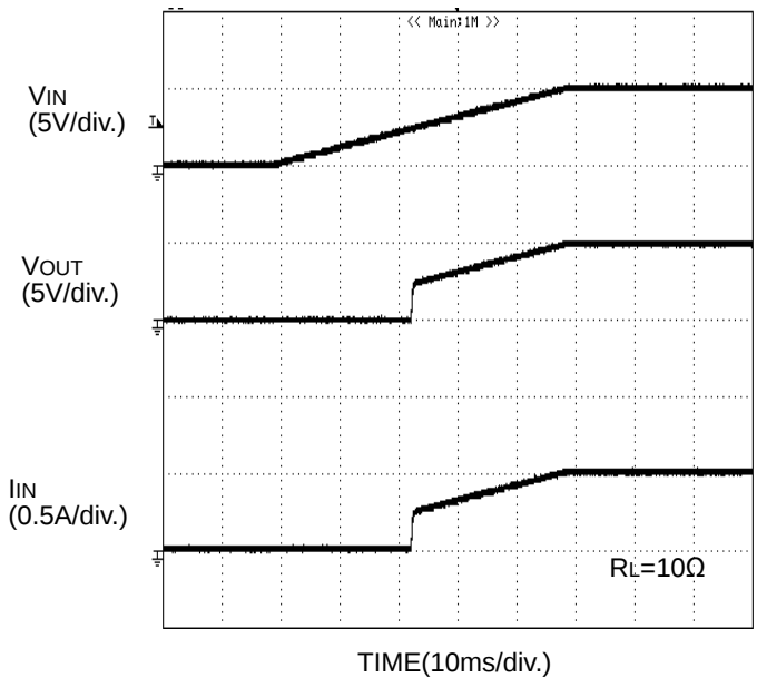
Figure 38. UVLO Response Increasing VIN
