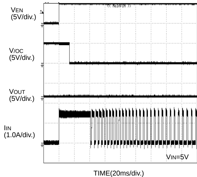
Figure 36. Over-Current Response Enable to Shortcircuit
