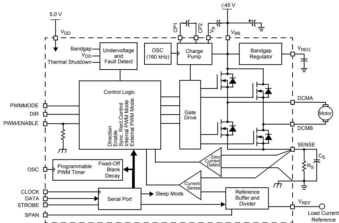
Figure 1. 34923 Simplified Block Diagram
