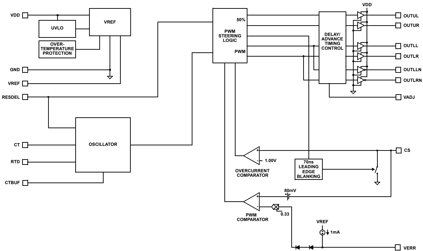
FIGURE 1. BLOCK DIAGRAM
