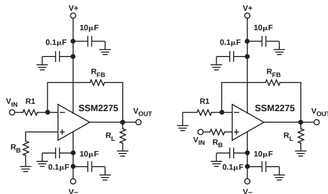
Figure 30. Basic Inverting and Noninverting Amplifiers
