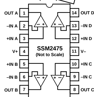
14-Lead Plastic DIP (N-14)
