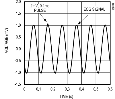
ECG PACEMAKER PULSE TOLERANCE 2mV, 0.1ms PULSE
