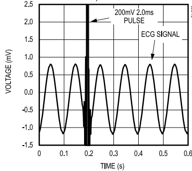
ECG PACEMAKER PULSE TOLERANCE 200mV, 2.0ms PULSE
