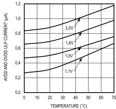
AVDD AND DVDD ULP CURRENT vs. TEMPERATURE
