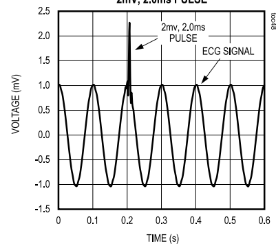
ECG PACEMAKER PULSE TOLERANCE 2mV, 2.0ms PULSE
