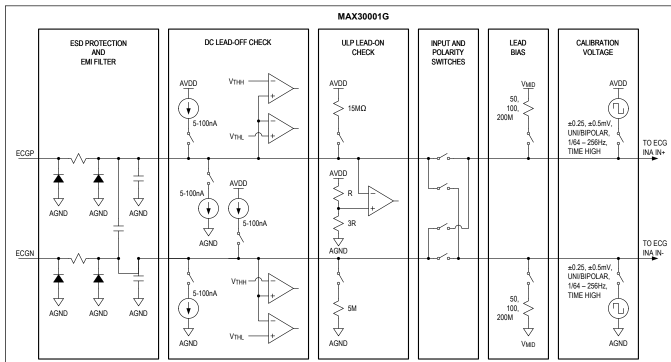
Figure 4. ECG Input MUX
