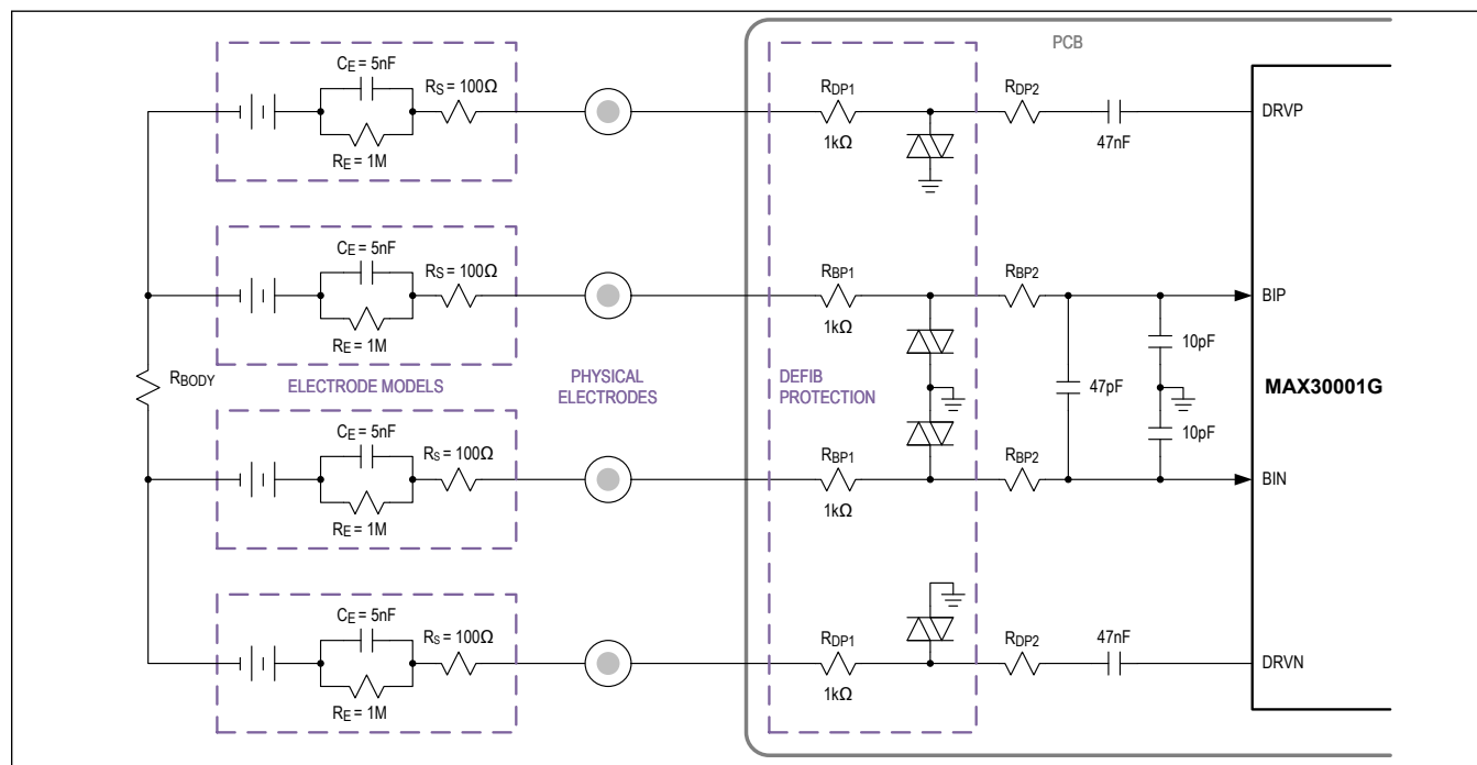
Figure 14. Example Configuration—Four Terminal
