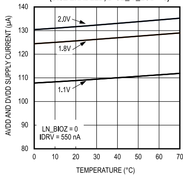
AVDD AND DVDD SUPPLY CURRENT vs. TEMPERATURE (BioZ ENABLED, BIOZ_HI_LOB = 0)
