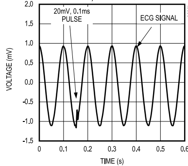
ECG PACEMAKER PULSE TOLERANCE 20mV, 0.1ms PULSE
