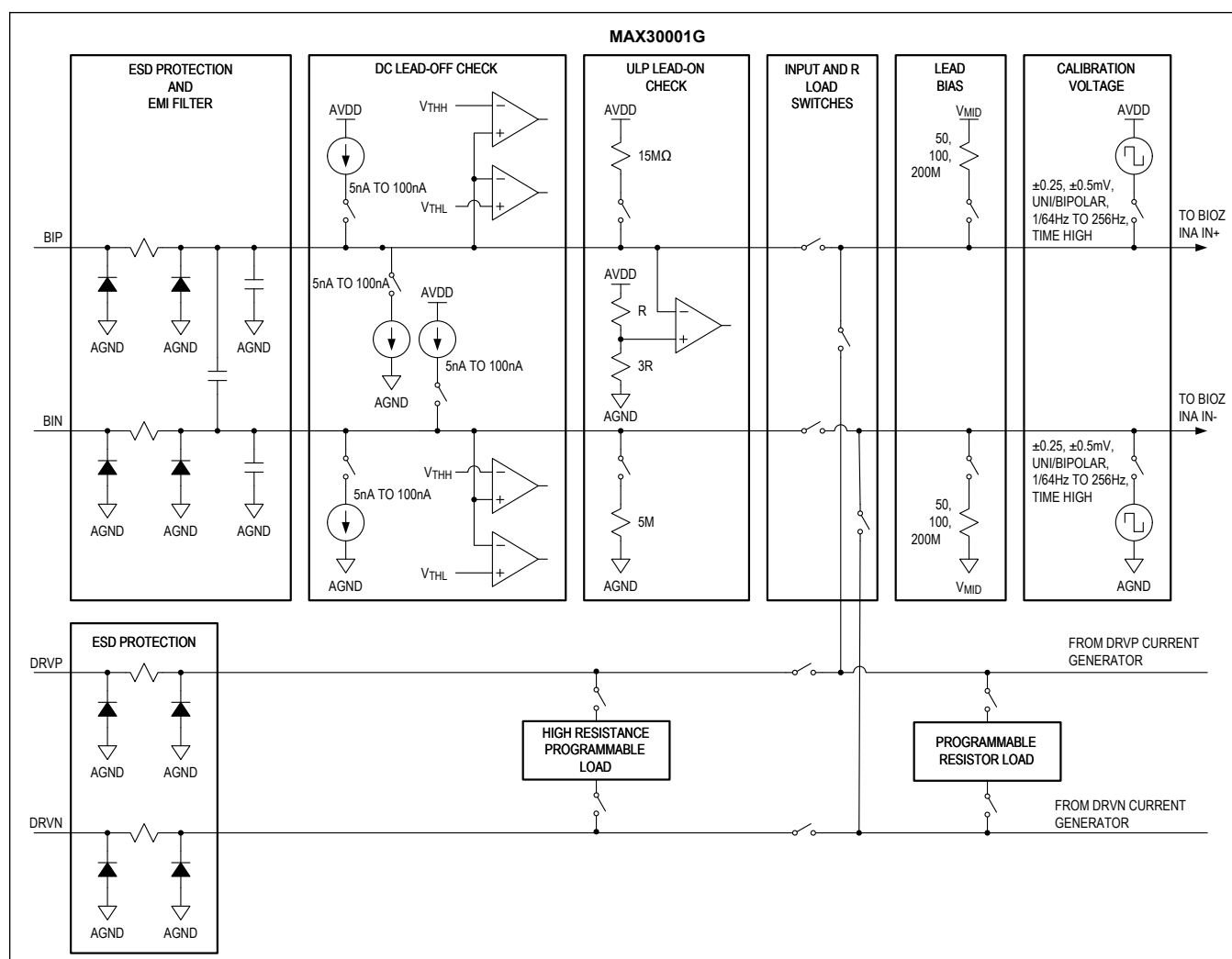
Figure 10. BioZ Input MUX
