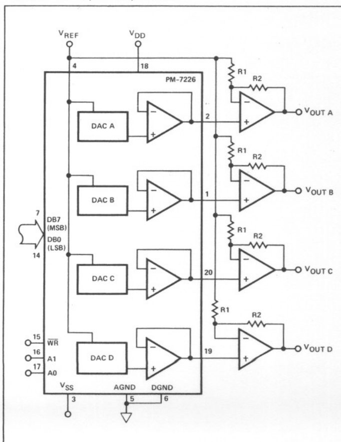
FIGURE 16: Bipolar Operation
