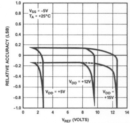
RELATIVE ACCURACY vs V_{REF}
