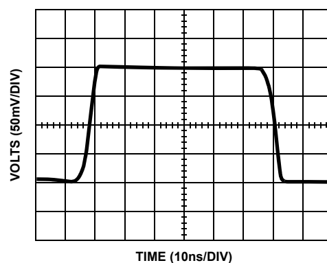
FIGURE 20. SMALL SIGNAL RISE &amp; FALL TIMES
