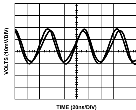
FIGURE 22. AMP OUTPUT NOISE (CHARGE PUMP OSCILLATION)
