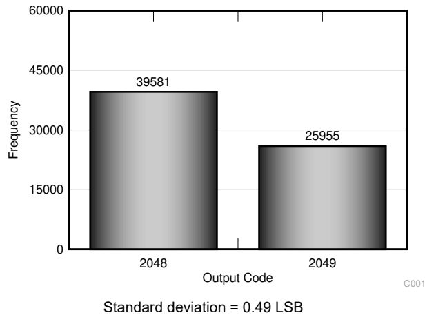
Figure 7-2. DC Input Histogram
