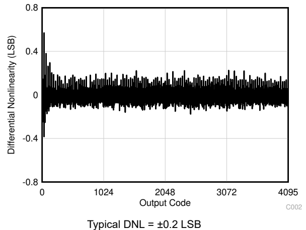
Figure 7-3. Typical DNL
